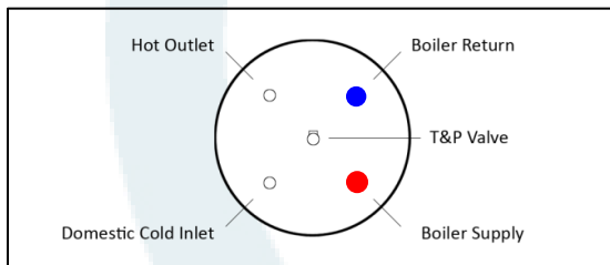
Top of Tank Connections
